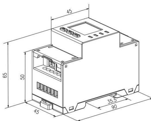
图 2 ADL400N-CT Figure 2 ADL400N-CT
