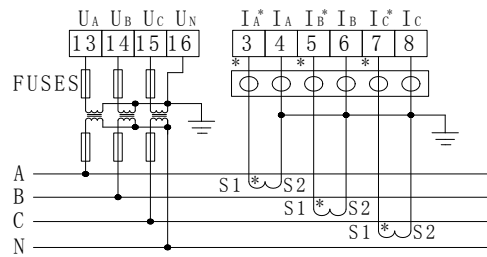
三相四线 3PT、3CT Three-phase 4-wire 3PT, 3CT
